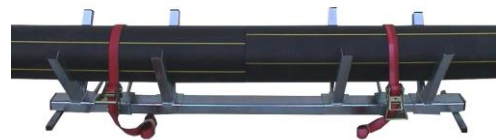
PM 160/450 - Manchon
